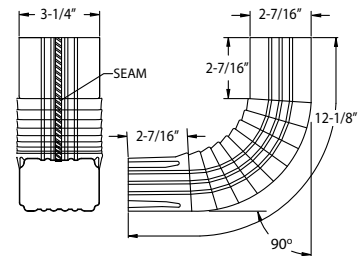
AAE923 A-Elbow
